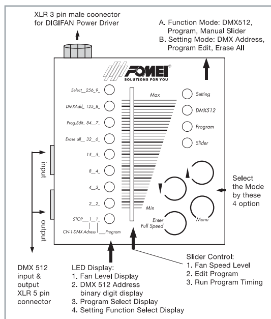
Operation-DMX Controller Box
